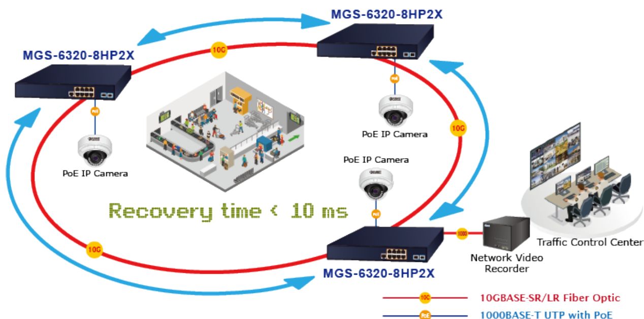
Figure 4-8-6-1: Ring Example Diagram
